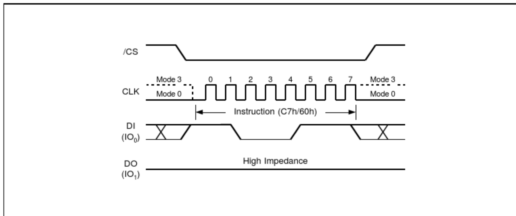
Figure 24. Chip Erase Instruction Sequence Diagram
